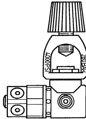
Bügel / YOKE
